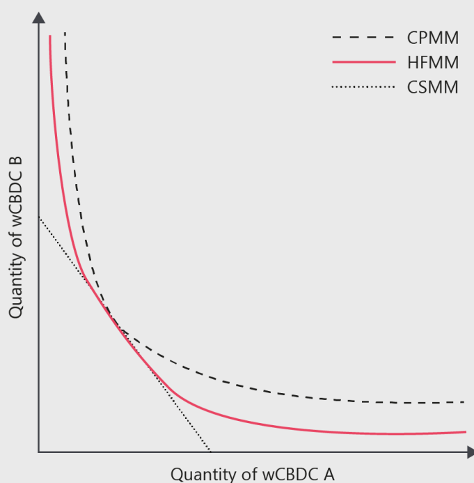
AMM bonding curve examples
